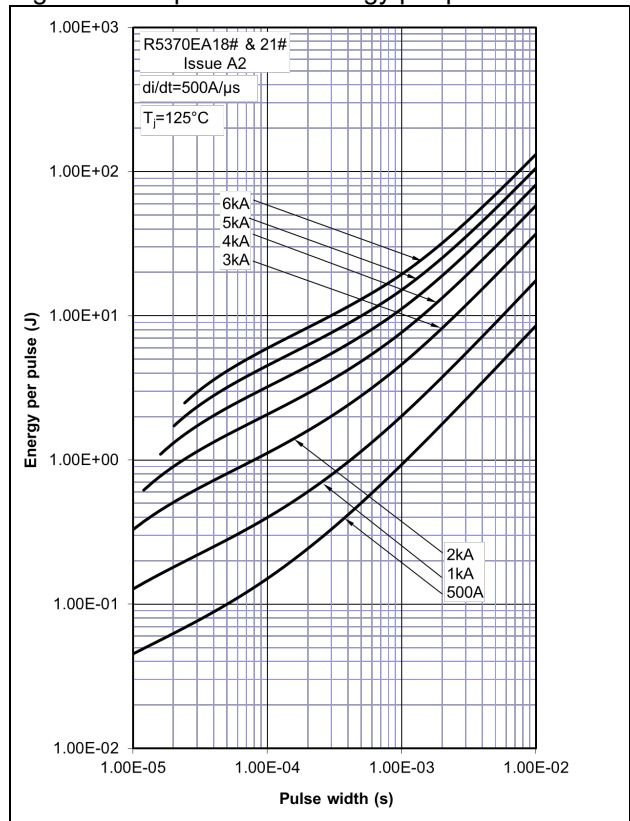
Figure 17 - Square wave energy per pulse
