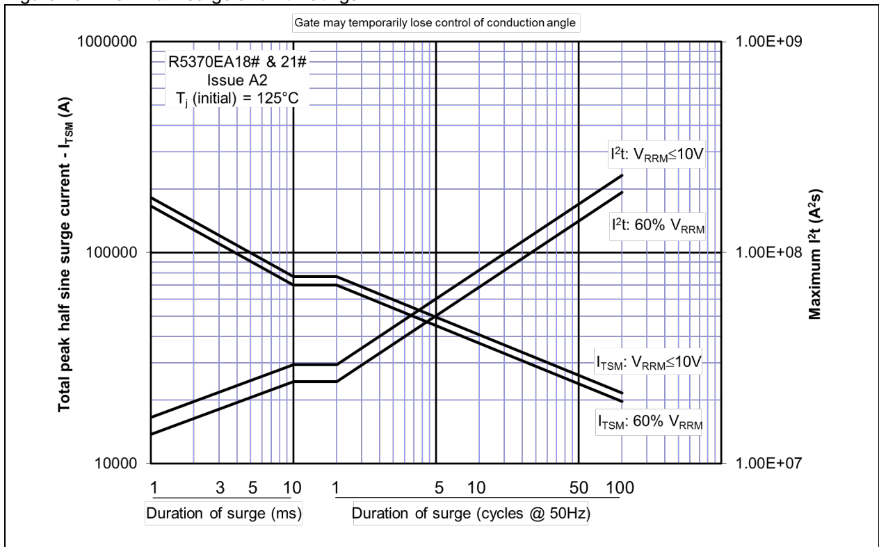
Figure 18 - Maximum surge and I^2t Ratings
