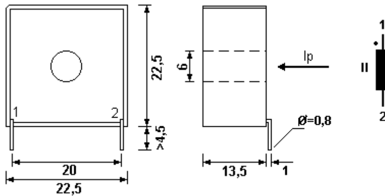
Pins side view Vista lato pin
