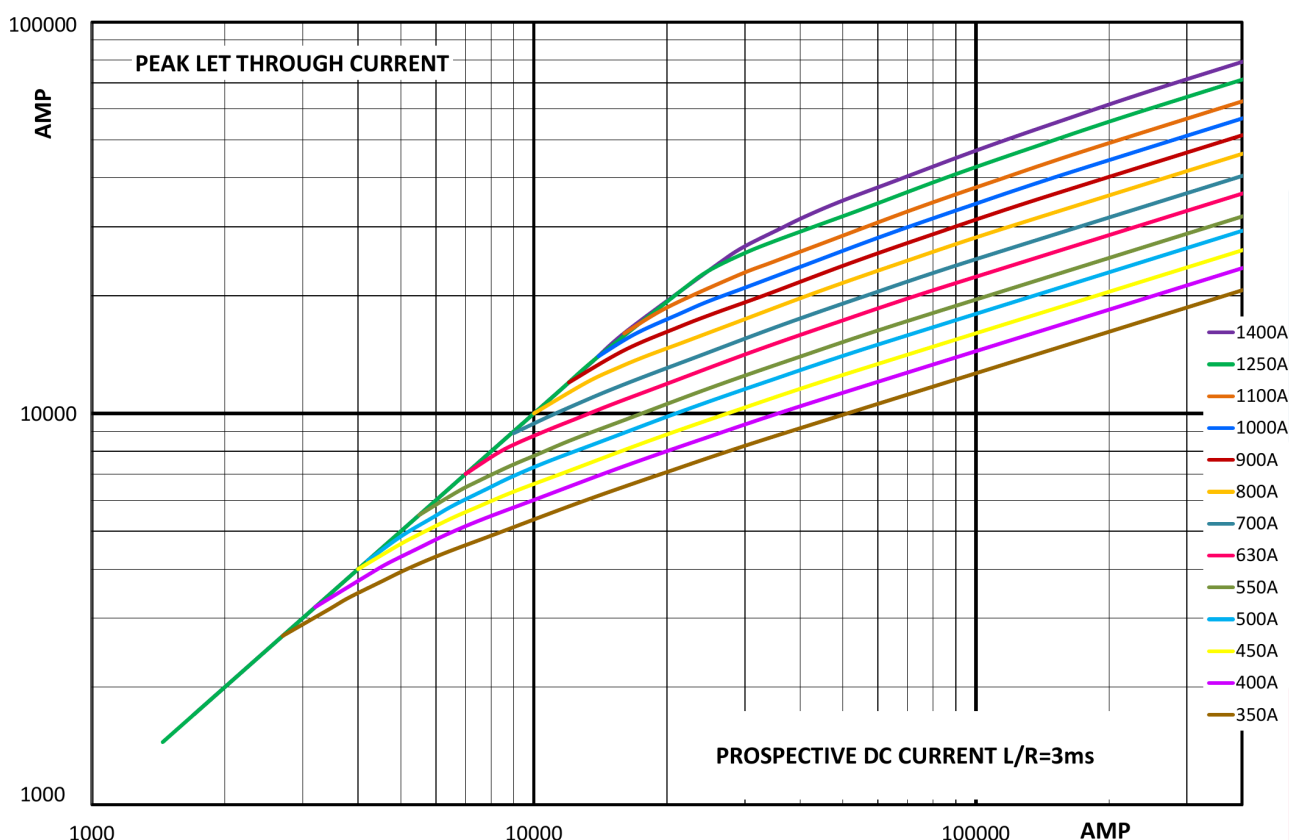
Figure 1. Eaton 180D size 3 peak let-through characteristic at 1,500 V DC and L/R = 3 ms [15].
